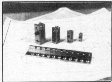
The tolerances of The Jointworks' ball-and-socket components are of a professional caliber, 1/10,000 of an inch. Machining is done on a computer-programmed, numerically-controlled mill.
